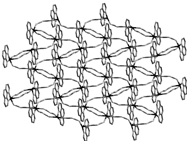
Fig. 10. The 2D (6,3) sheet topology of M(dca)_2(1,10\text{-phen}) , M = \text{Cu, Cd} .
